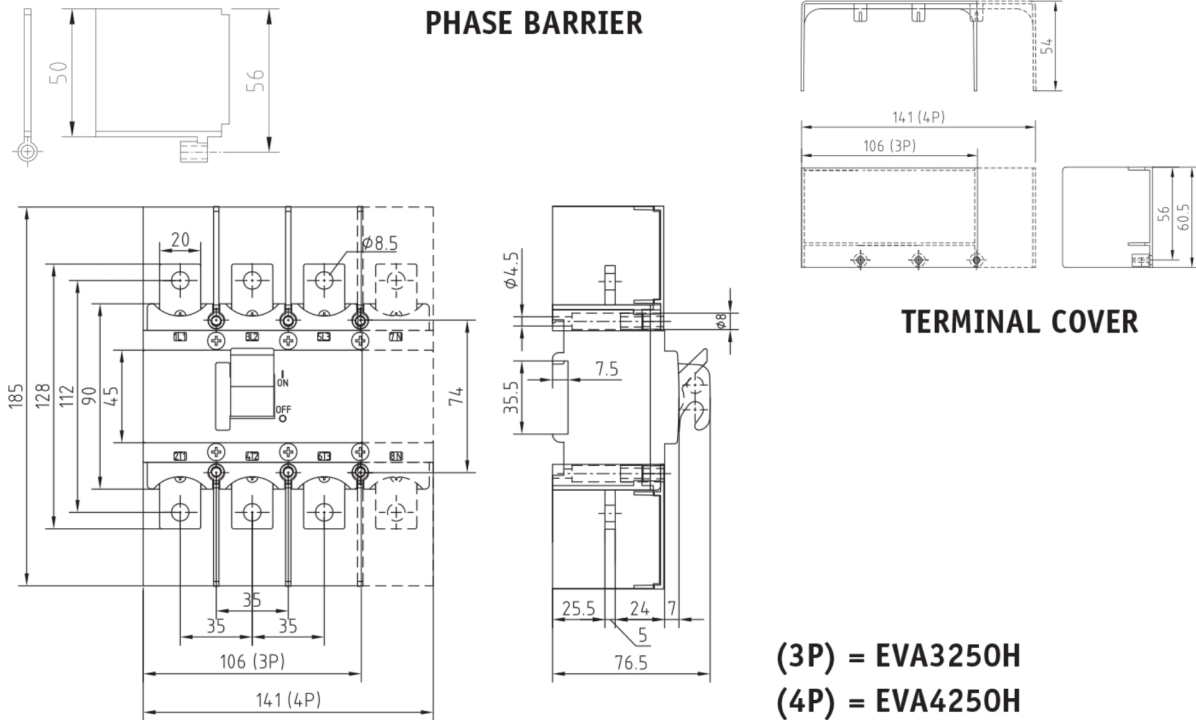
Dimension Diagram
