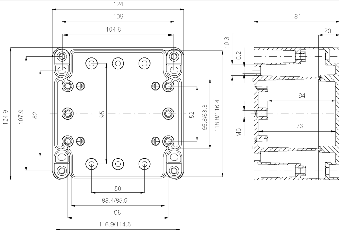
Dimension Diagram
