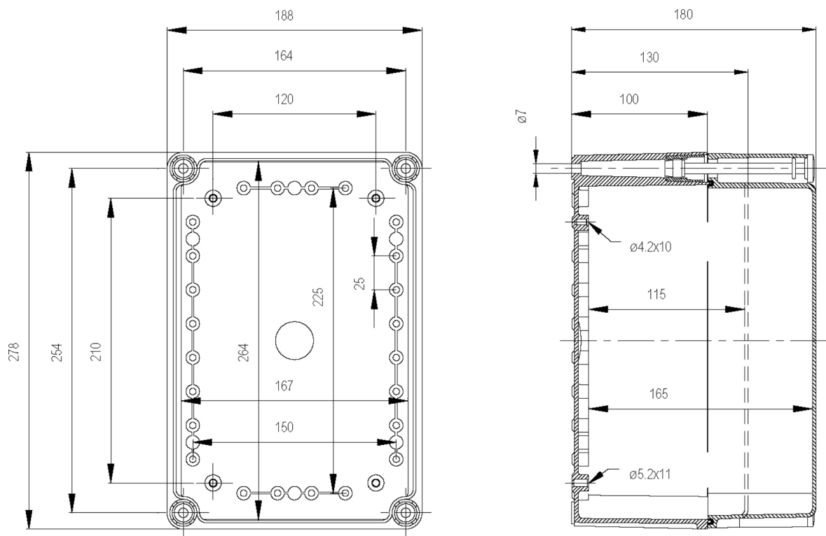
Dimension Diagram
