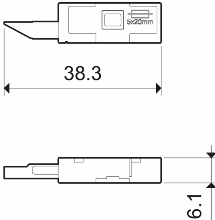
Dimension Diagram
