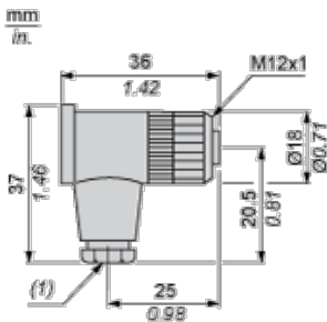
(1) Cable gland : no. 7 plastic (Pg 7)
