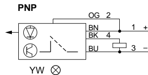
PNP
