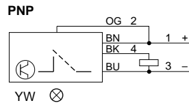
PNP
