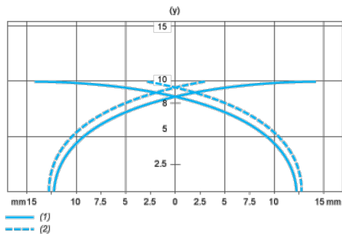
Standard Steel Target : 30x30x1 mm
