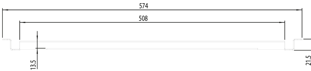
Dimension Diagram
