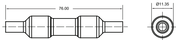
In-line with crimp terminals PV-(amp)A10F-CT (1-20A), PV10M(amp)A-CT (25-30A)
