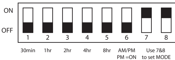
ECO Mode, 50% : 25% : 25% Setting
