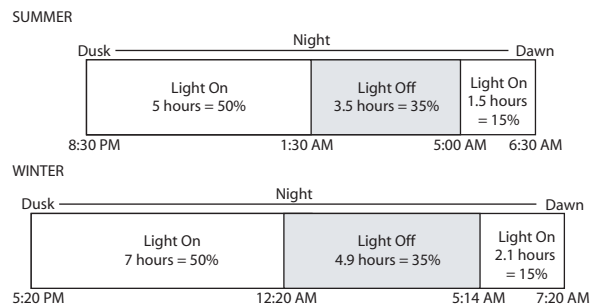
ECO mode: Switch 7 OFF (down) & Switch 8 ON (up)
