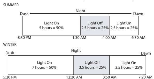
ECO mode: Switch 7 ON (up) & Switch 8 ON (up)
