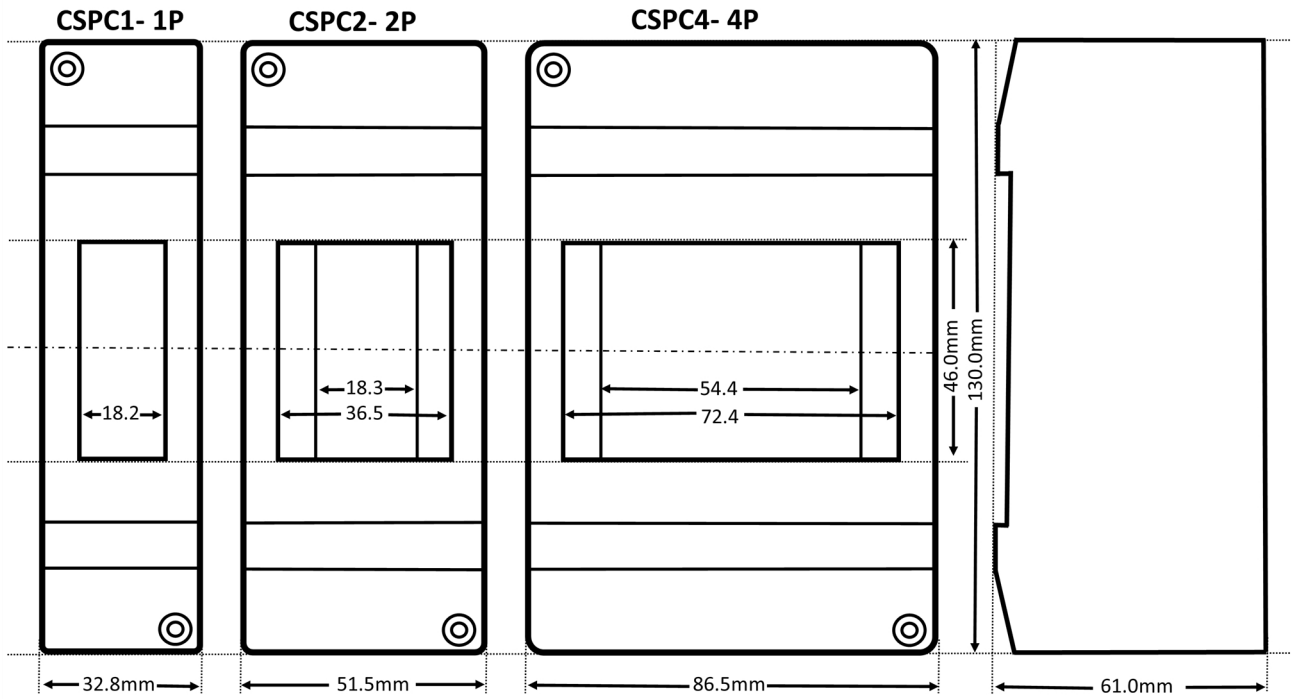
Dimension Diagram
