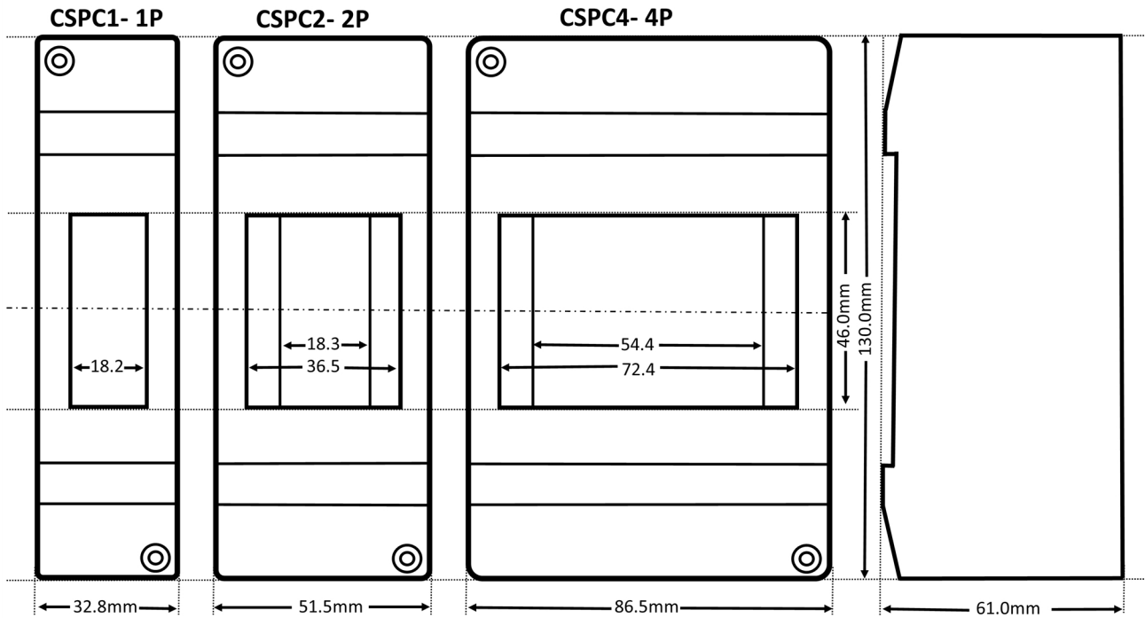
Dimension Diagram
