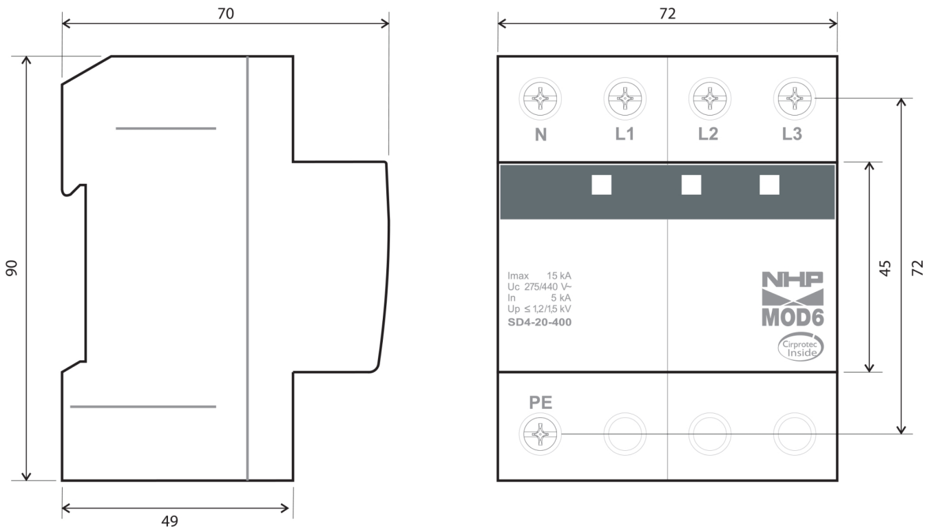
Dimension Diagram
