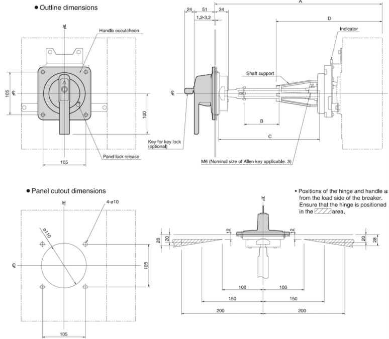
Dimension Diagram
