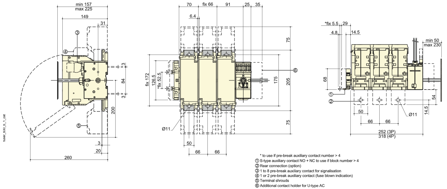
Dimension Diagram
