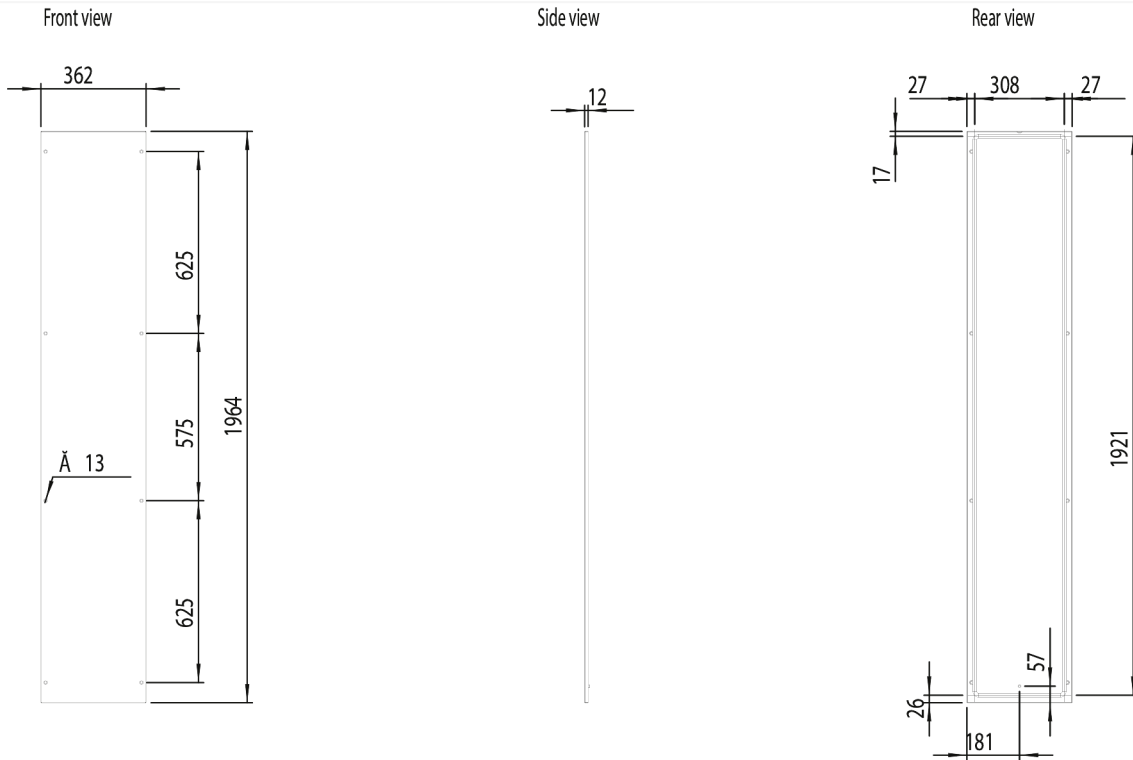
Dimension Diagram
