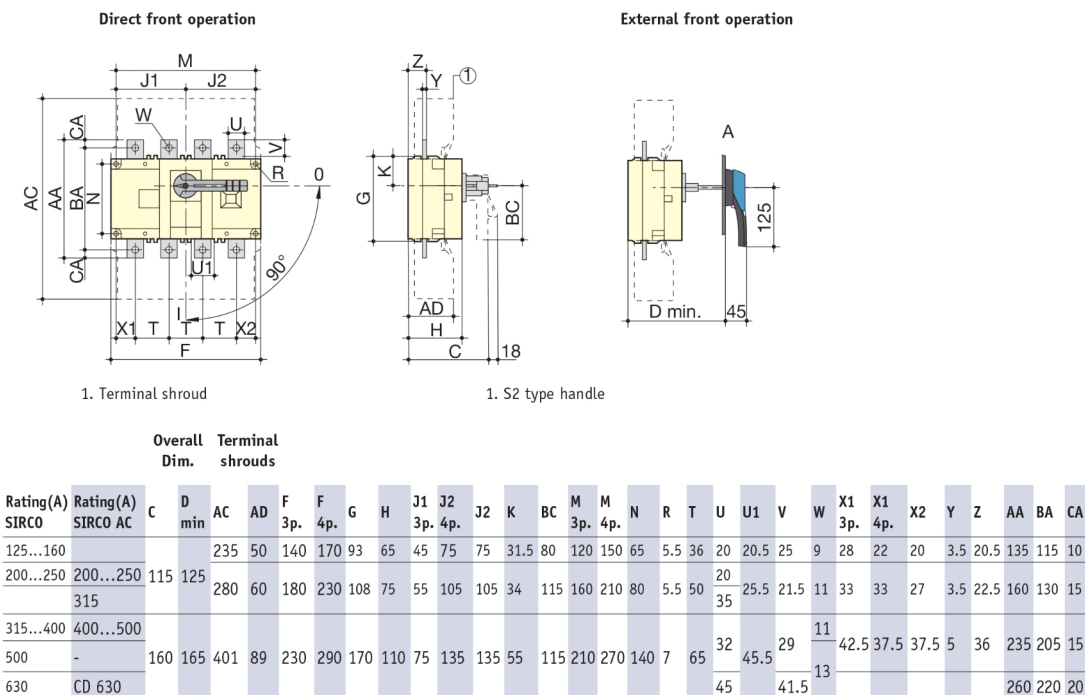
Dimension Diagram
