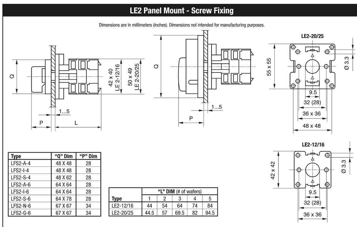
Dimension Diagram
