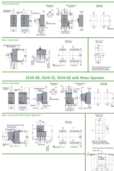
Dimension Diagram
