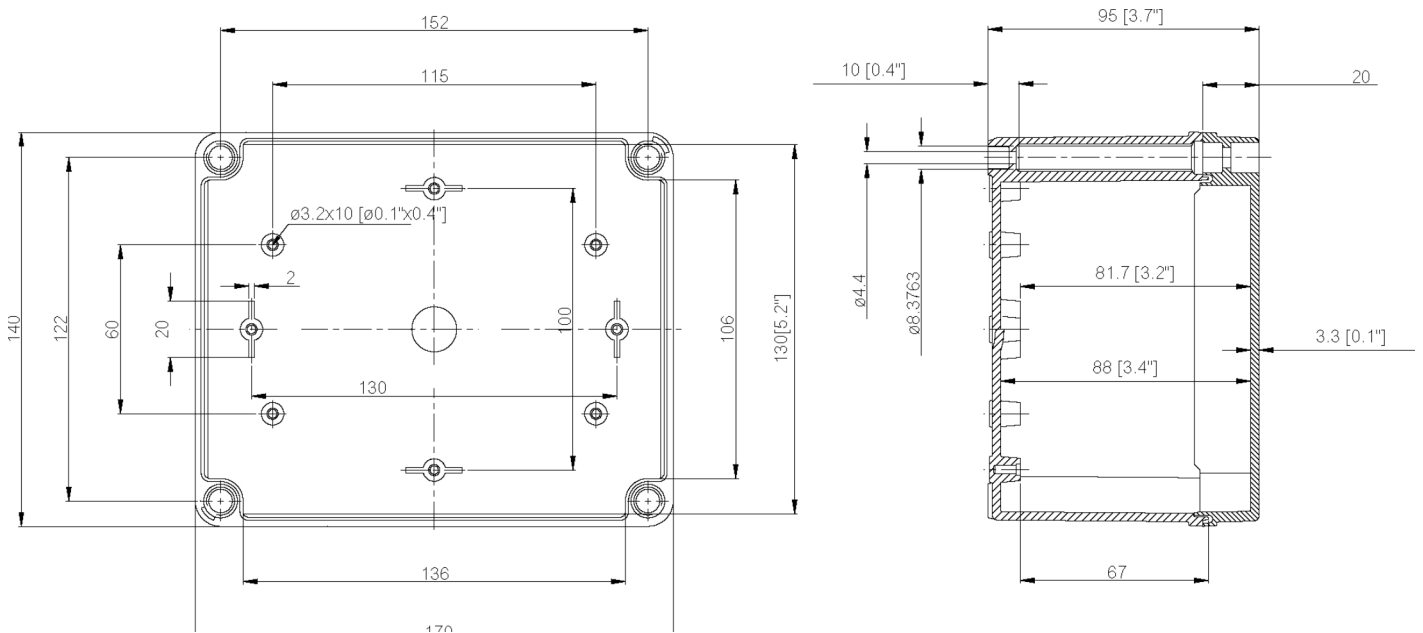
Dimension Diagram
