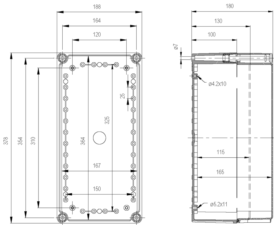
Dimension Diagram
