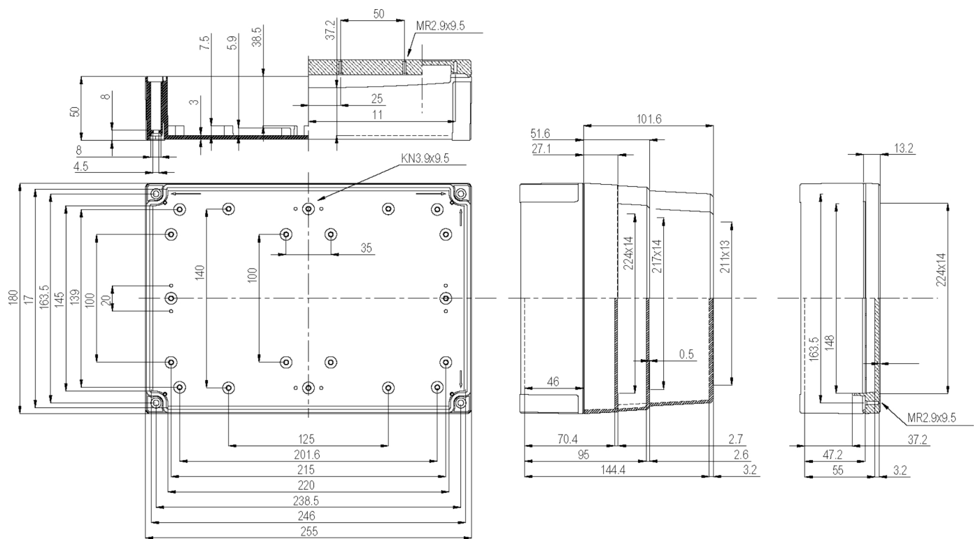
Dimension Diagram
