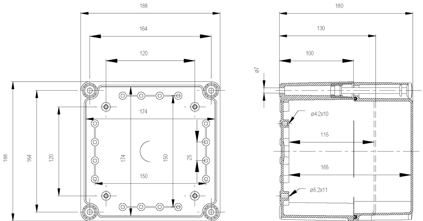
Dimension Diagram
