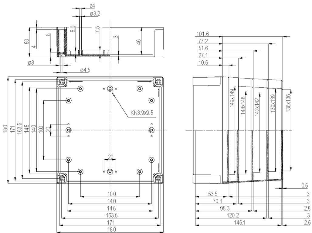
Dimension Diagram
