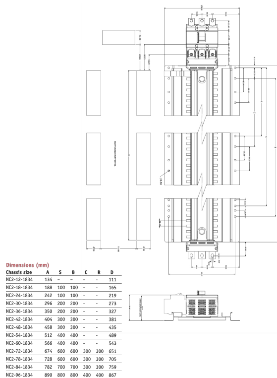
Dimension Diagram
