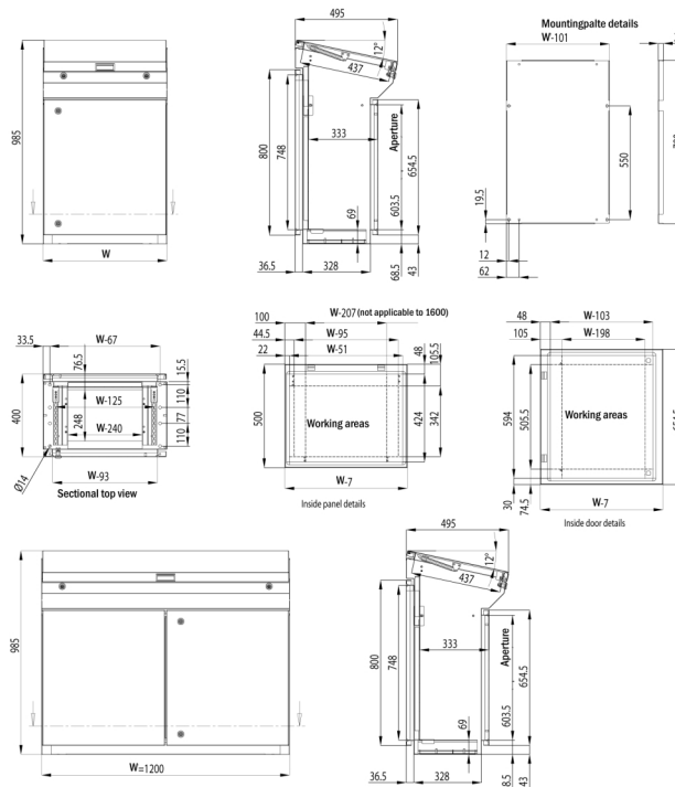
Dimension Diagram
