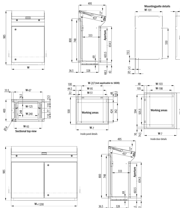
Dimension Diagram
