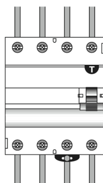
4 P (240/415 V)
