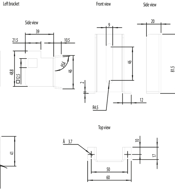
Dimension Diagram
