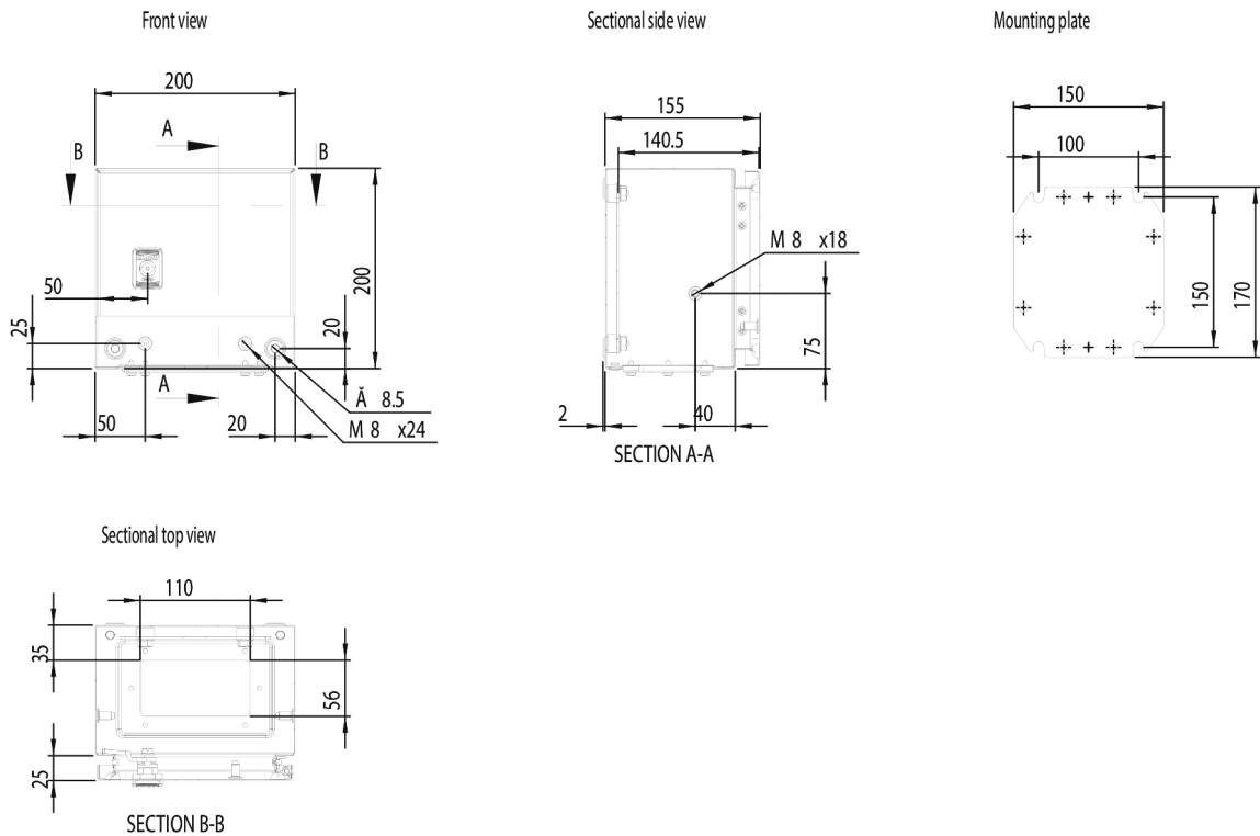
Dimension Diagram
