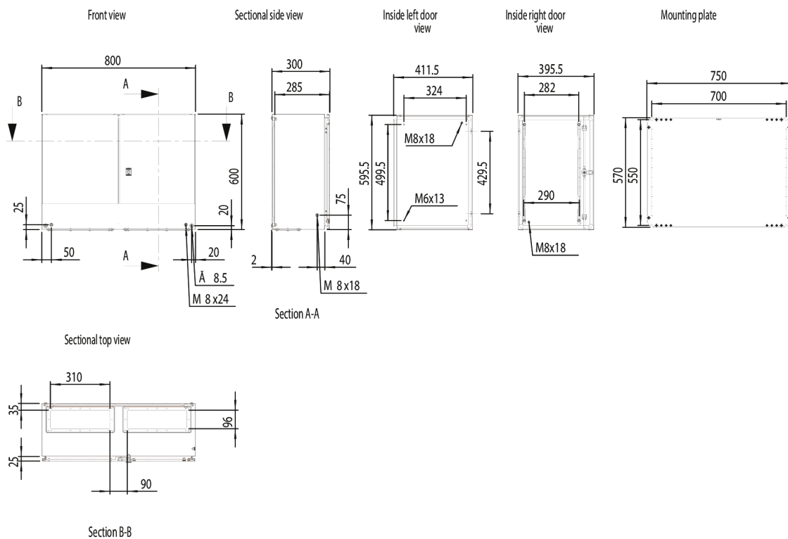
Dimension Diagram
