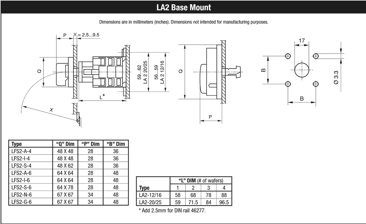
Dimension Diagram
