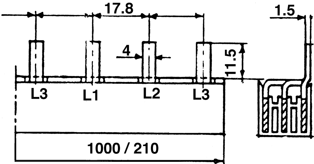
Dimension Diagram
