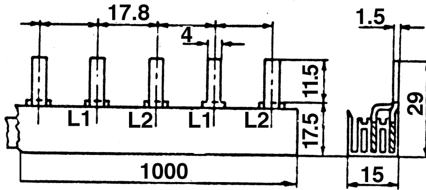
Technical Diagram
