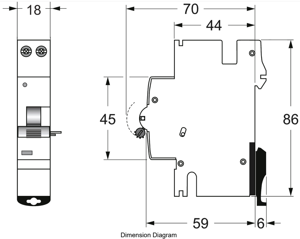
Dimension Diagram
