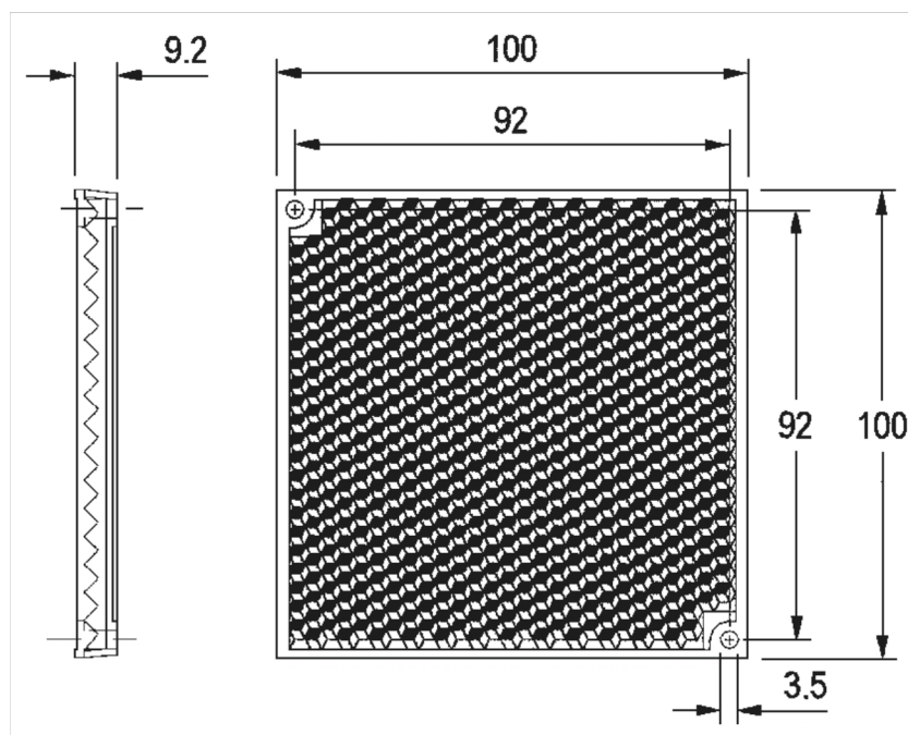
Dimension Diagram
