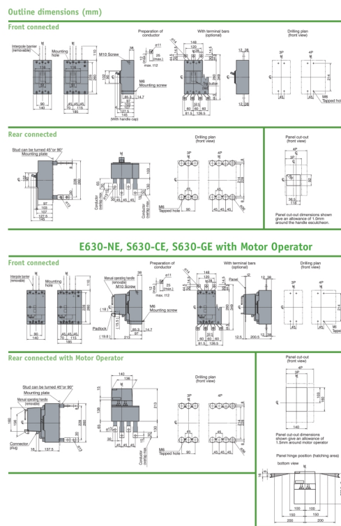
Dimension Diagram
