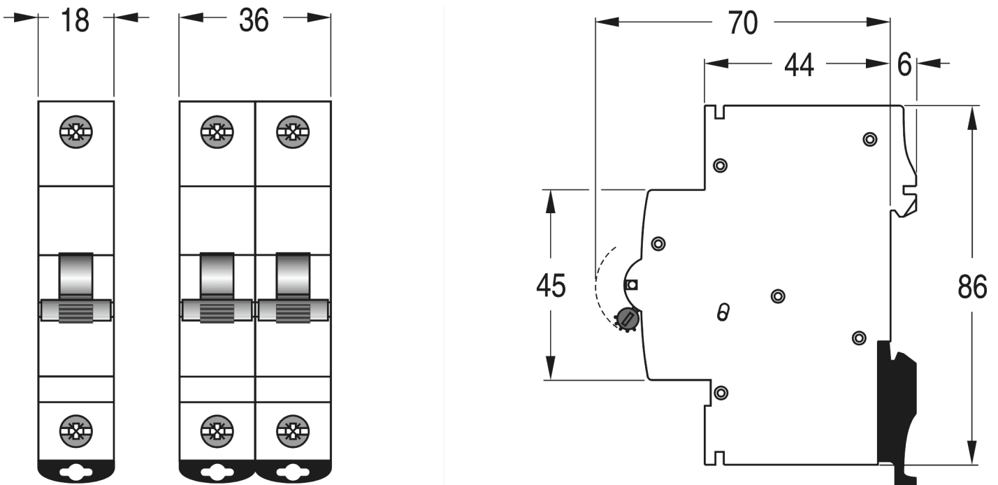
Dimension Diagram
