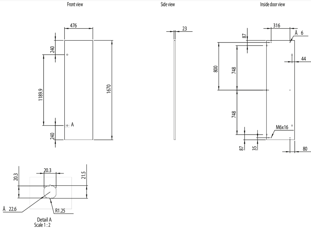
Dimension Diagram
