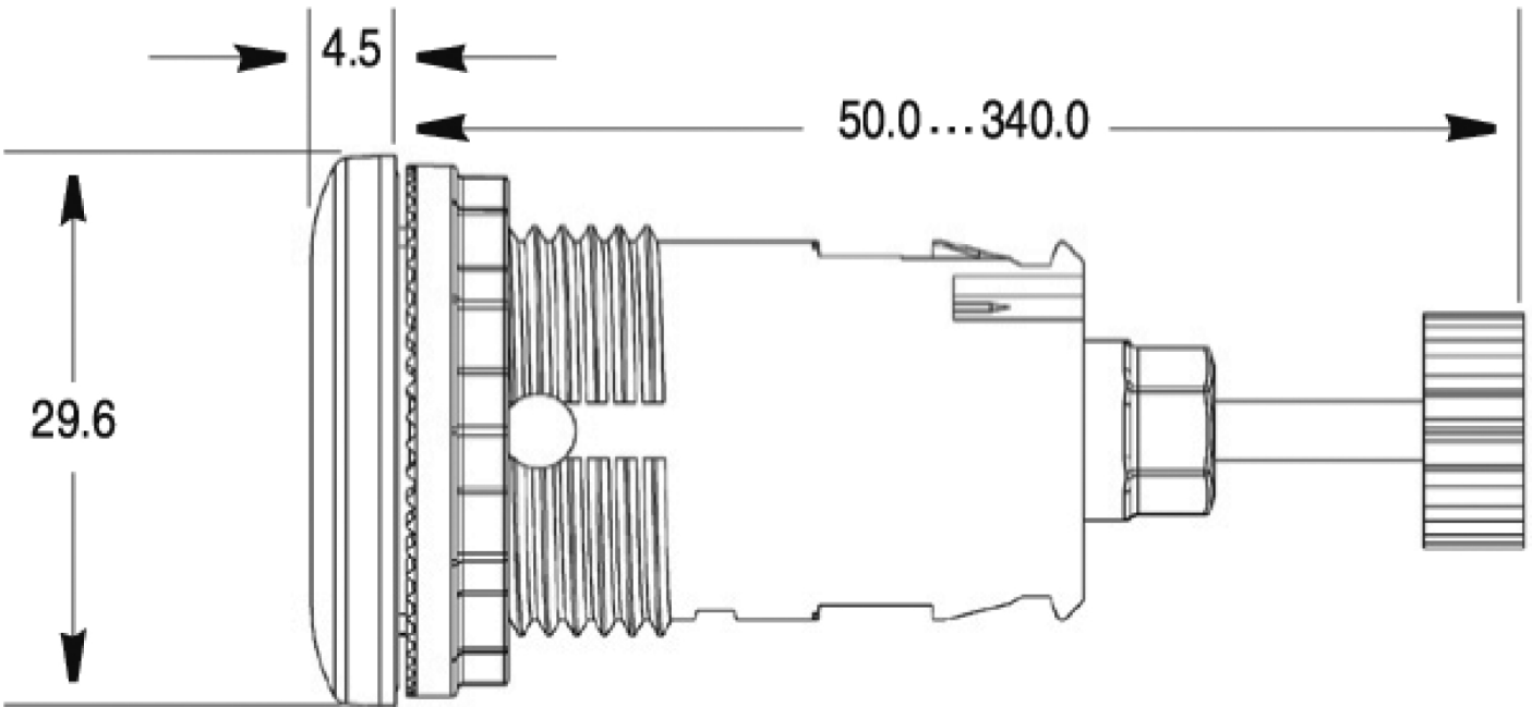
Dimension Diagram
