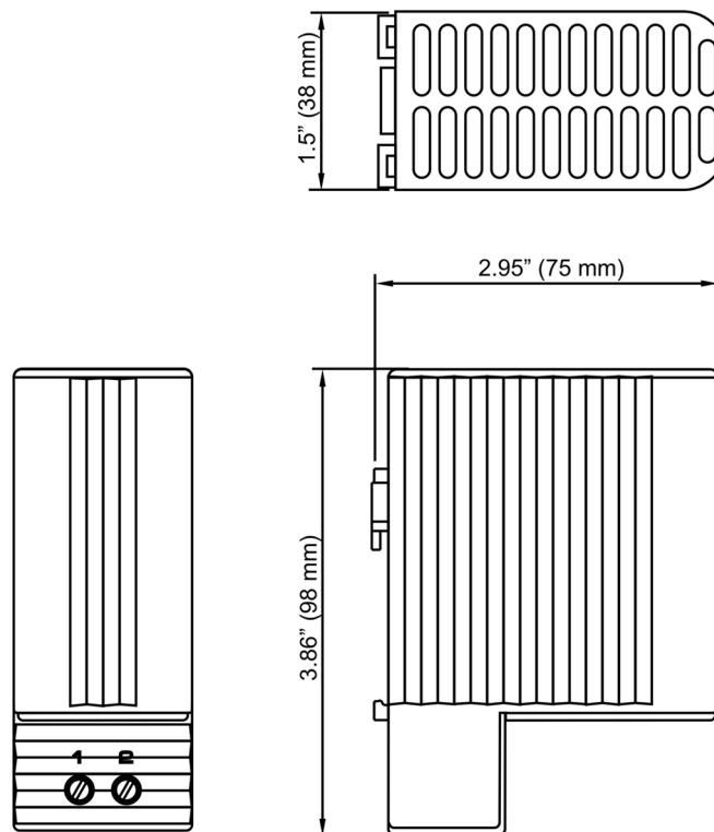
Dimension Diagram
