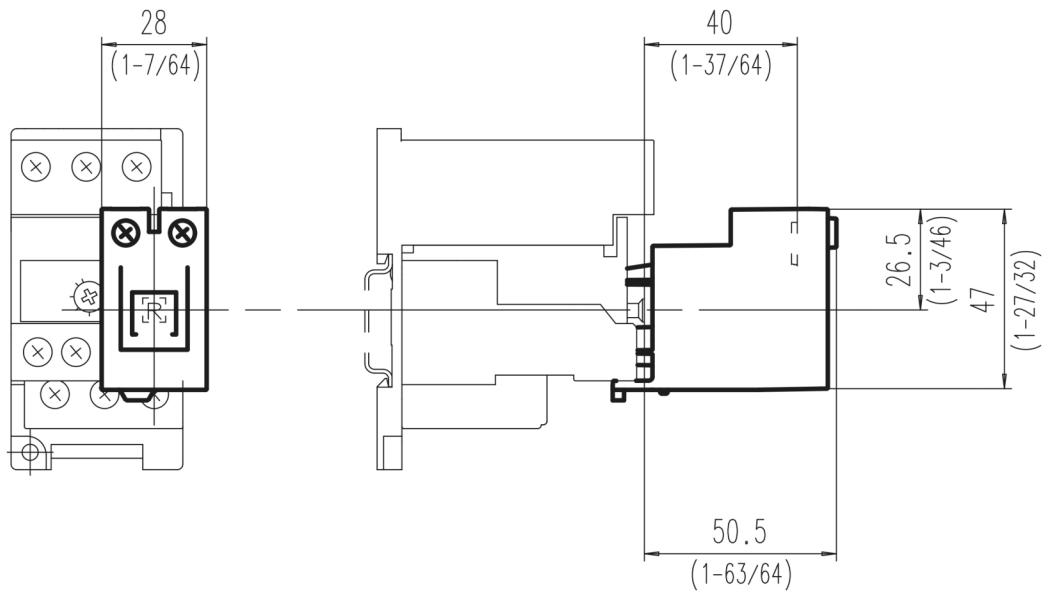
Dimension Diagram
