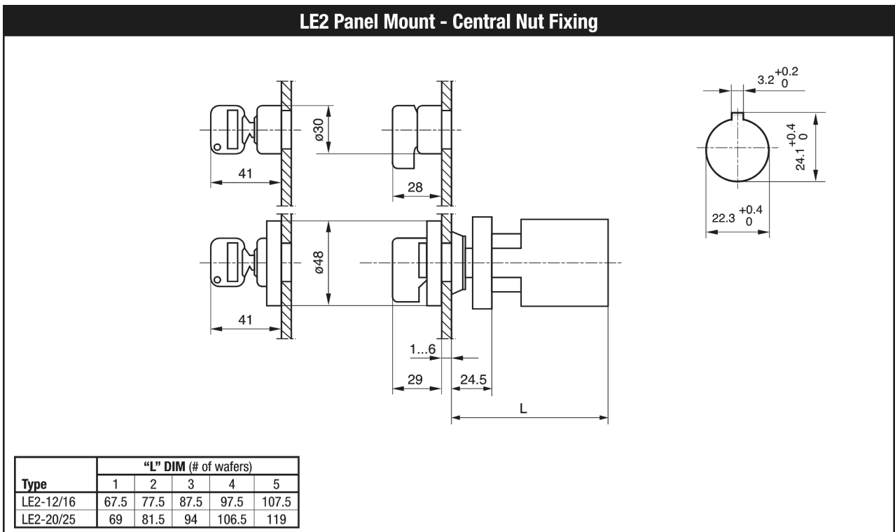
Dimension Diagram
