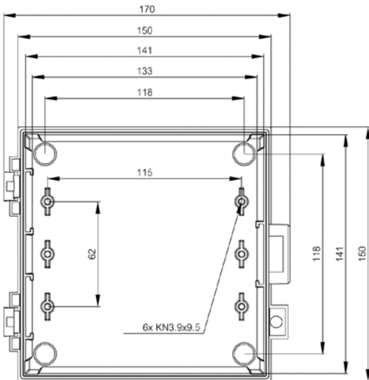
Dimension Diagram
