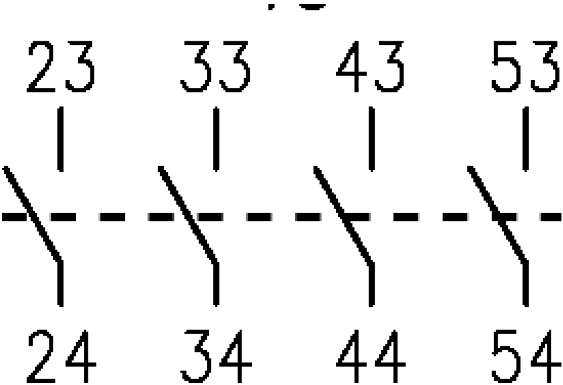
Connection / Wiring Diagram
