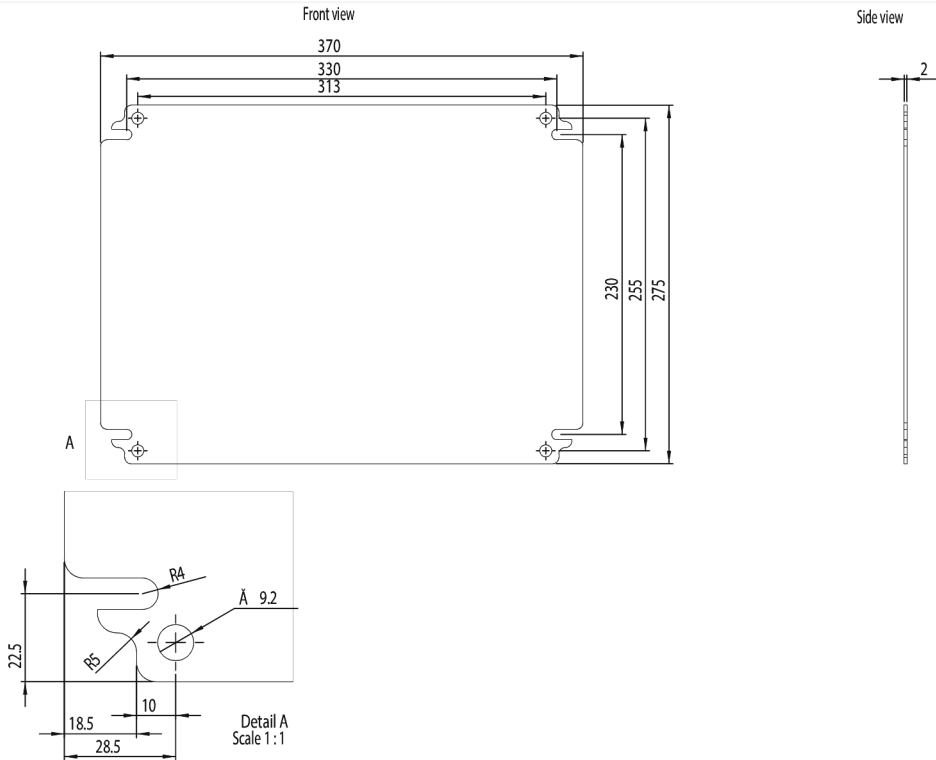
Dimension Diagram
