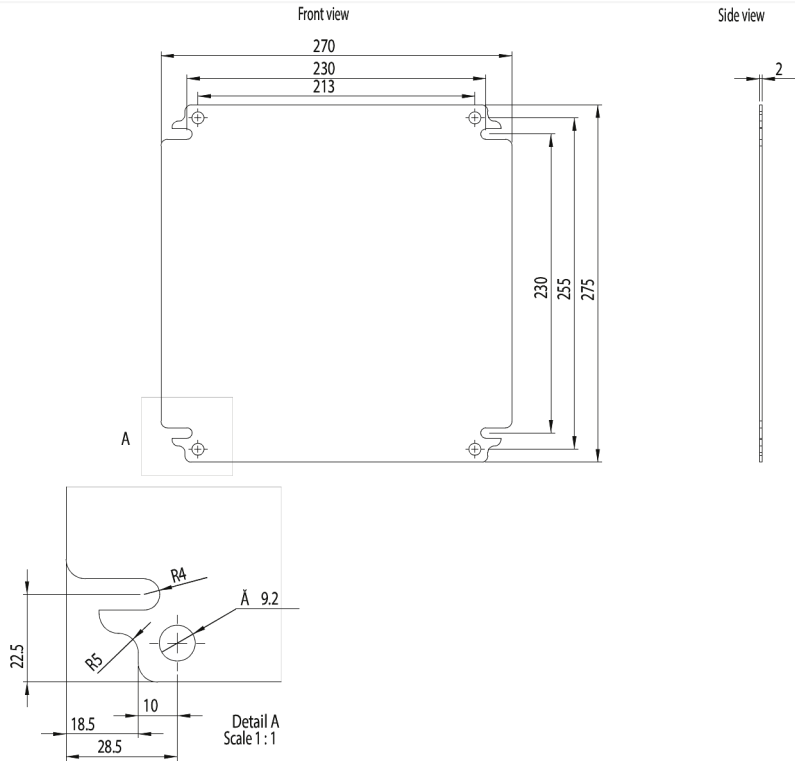
Dimension Diagram
