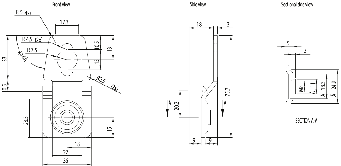
Dimension Diagram
