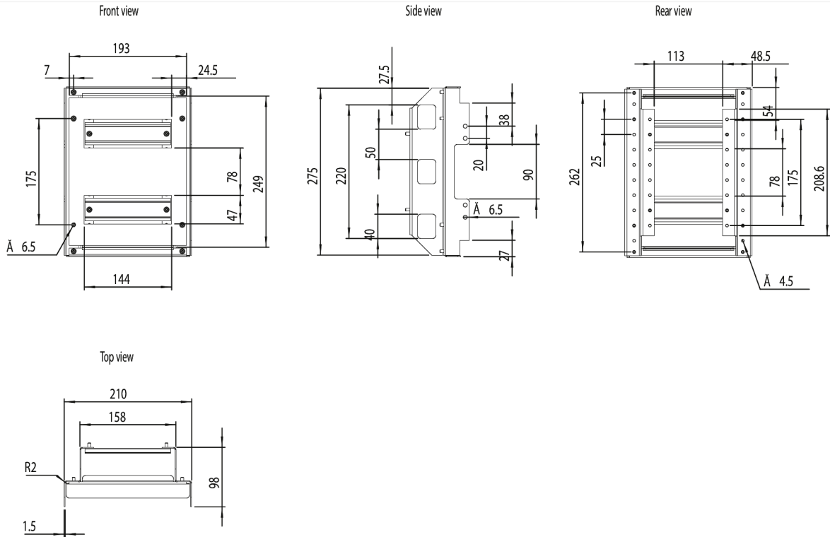
Dimension Diagram
