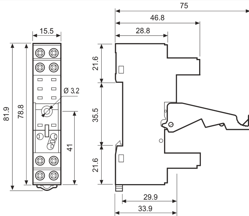
Dimension Diagram
