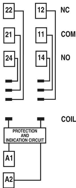
93.02/52 Connection / Wiring Diagram
